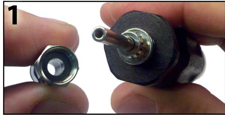
1 Hold the F Connector and CGT-FBR Tool in each hand
