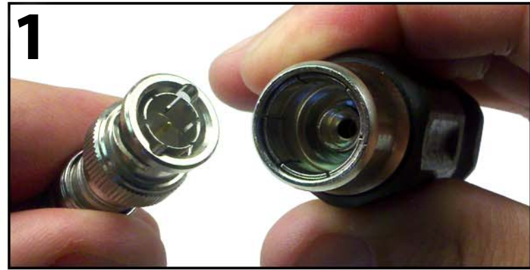
Hold the BNC Connector and CGT-FBR Tool in each hand
