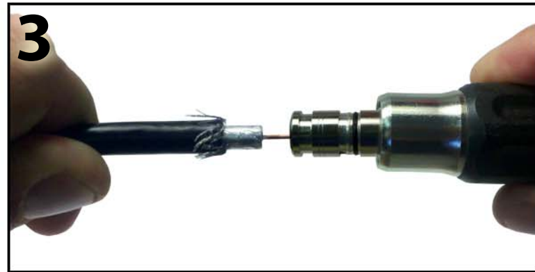
Guide your stripped coax into the end of the RCA connector
