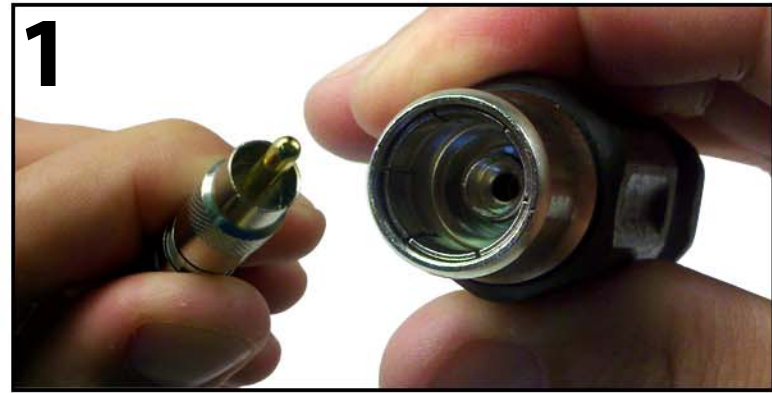
Hold the RCA Connector and CGT-FBR Tool in each hand
